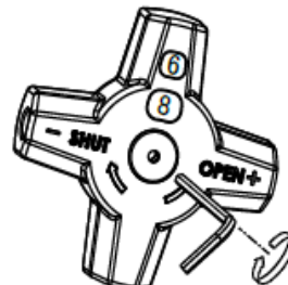
锁定位置 Lock position 锁定位置为6.8圈 The locked presetting value is 6.8 turns
