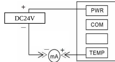
Current Output 2-wire Connecting
