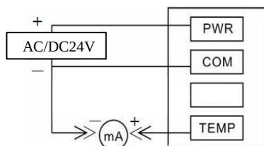
Current Output 3-wire Connecting
