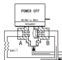
Fig.5:3-way valve in Diverting Configuration, Normally Open to coil
