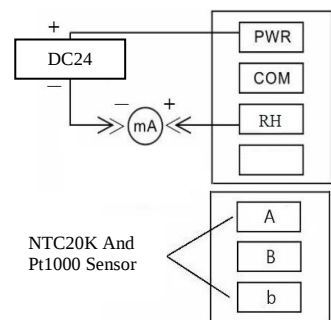
Current Output 2-wire Connecting
