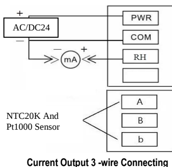
Current Output 3-wire Connecting
